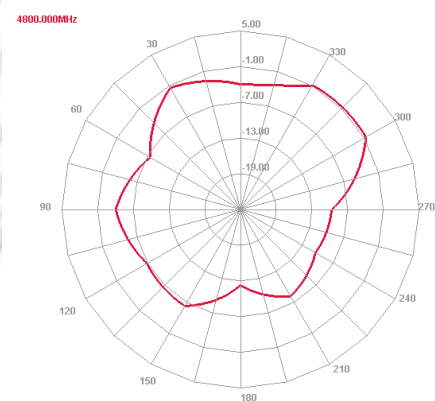
Horizontal
