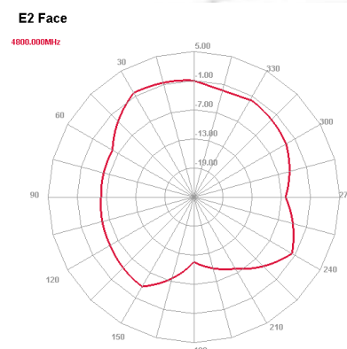
4800 MHz E plane
