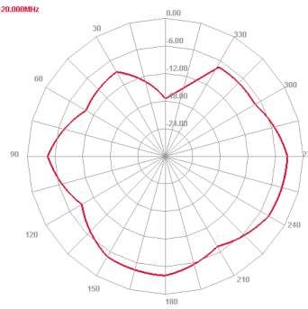
7120 MHz H plane
