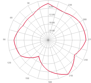
5800 MHz H plane
