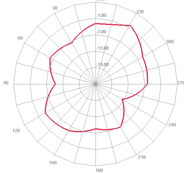
5800 MHz E plane
