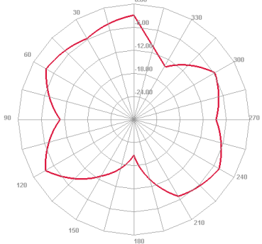
7120 MHz E plane
