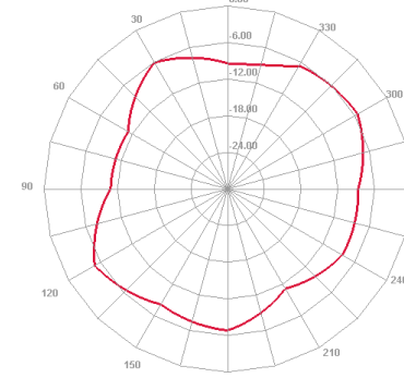
7120 MHz H plane
