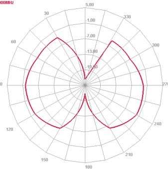
6000 MHz E plane
