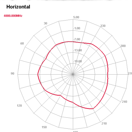
4800 MHz H plane
