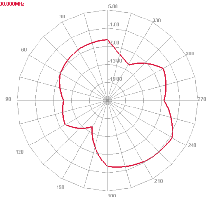
4800 MHz H plane
