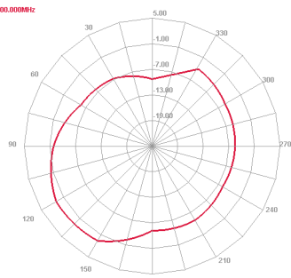
2600 MHz H plane
