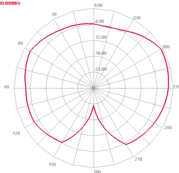
5800 MHz E plane
