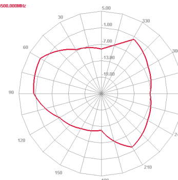
3500 MHz E plane
