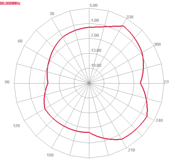
2400 MHz H plane
