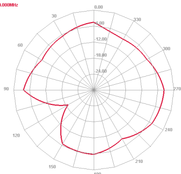
800 MHz E plane
