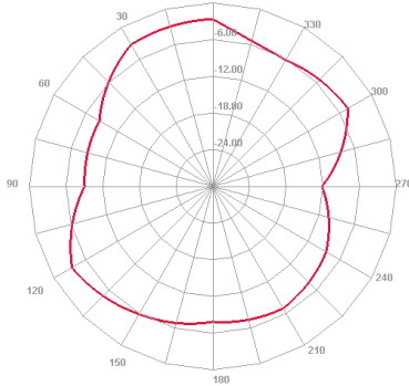
6000 MHz E plane
