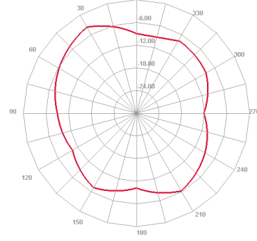
6000 MHz H plane
