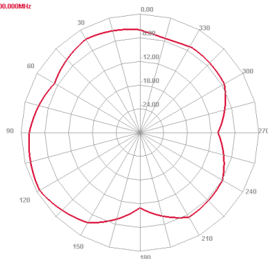
2100 MHz E plane
