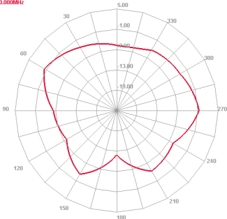
2600 MHz E plane
