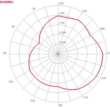
3500 MHz H plane
