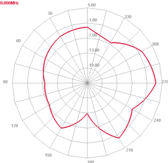
3500 MHz E plane
