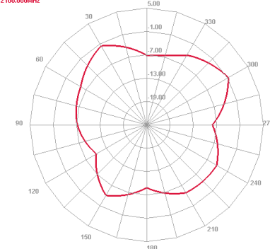
Horizontal
