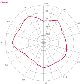
Horizontal
