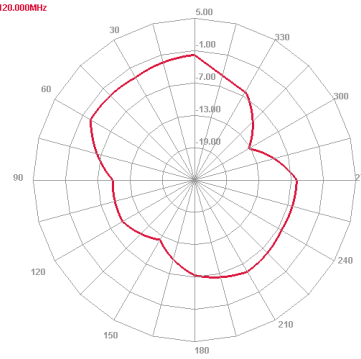
7120 MHz H plane
