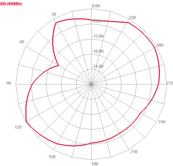
1800 MHz H plane
