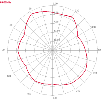
5800 MHz E plane
