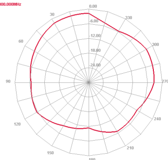
1800 MHz E plane
