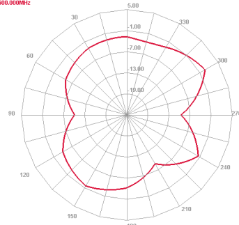
2600 MHz H plane
