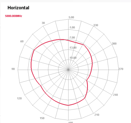
5800 MHz H plane
