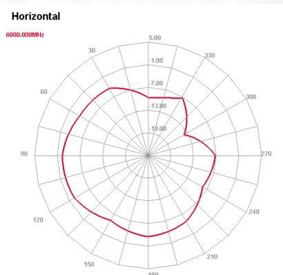
6000 MHz H plane
