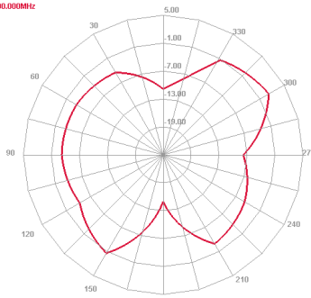
2600 MHz H plane
