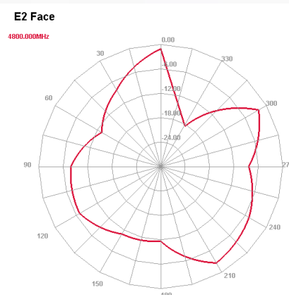
4800 MHz E plane
