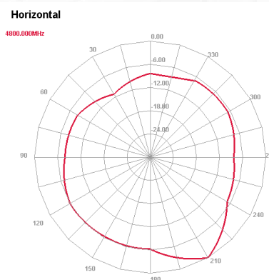
4800 MHz H plane
