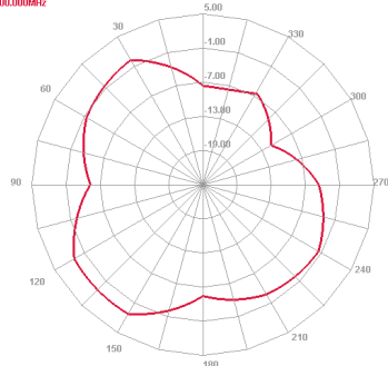
2400 MHz H plane
