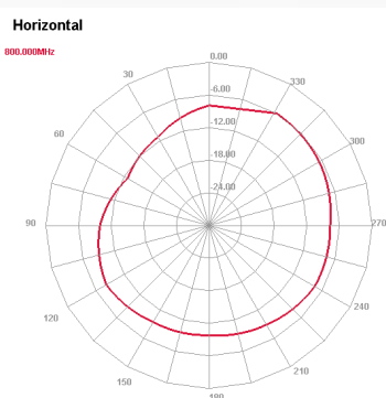
800 MHz H plane
