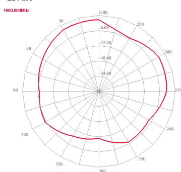
1800 MHz E plane
