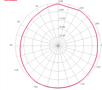
900 MHz H plane
