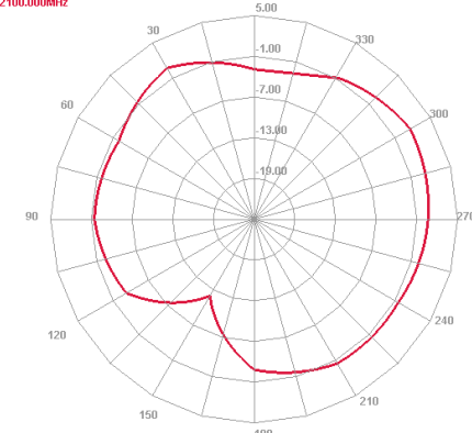
2100 MHz H plane
