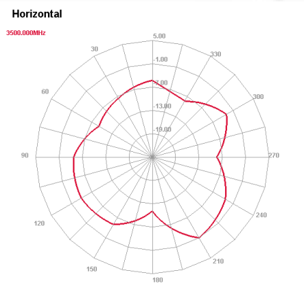
3500 MHz H plane
