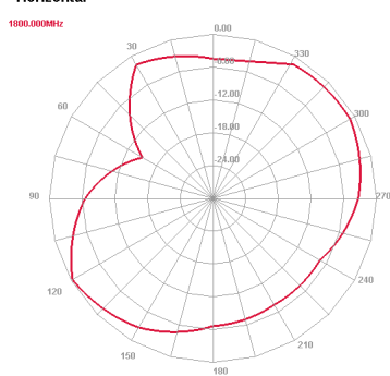
1800 MHz H plane
