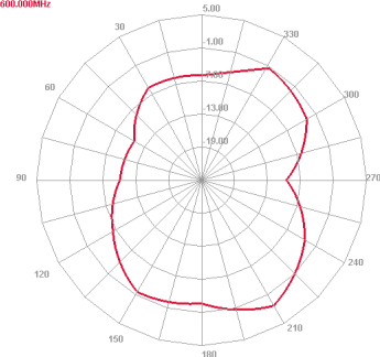
2600 MHz E plane
