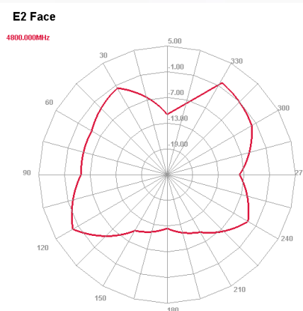
4800 MHz E plane
