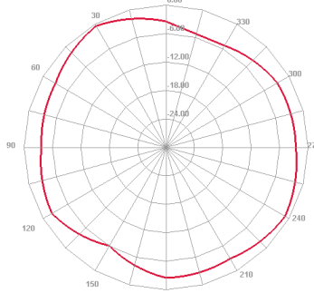
900 MHz E plane
