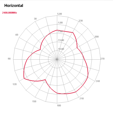
2400 MHz H plane
