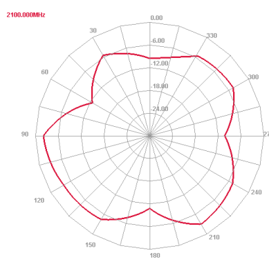
2100 MHz H plane
