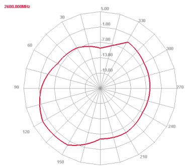
2600 MHz H plane
