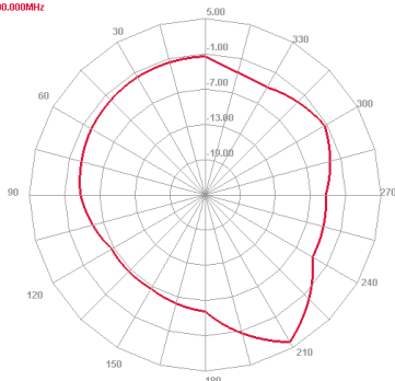
2600 MHz E plane
