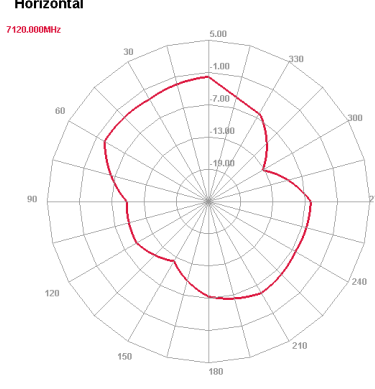
7120 MHz H plane
