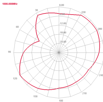
1800 MHz H plane
