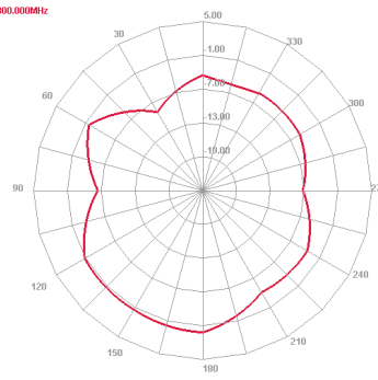
5800 MHz H plane
