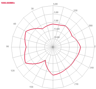
1800 MHz H plane
