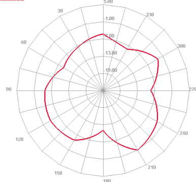
3500 MHz E plane
