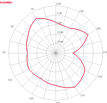
2400 MHz E plane
