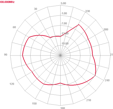
2100 MHz H plane
