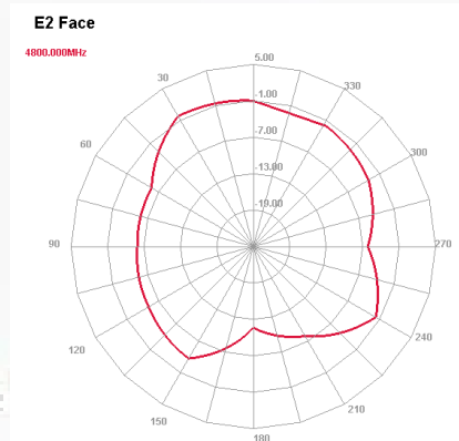
4800 MHz E plane
