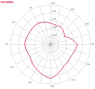
1800 MHz E plane
