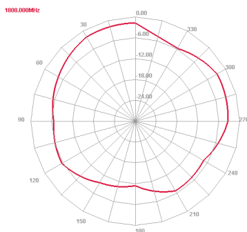
1800 MHz E plane
