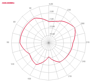
2600 MHz E plane
