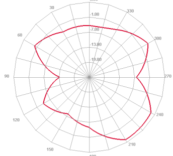
2600 MHz E plane
