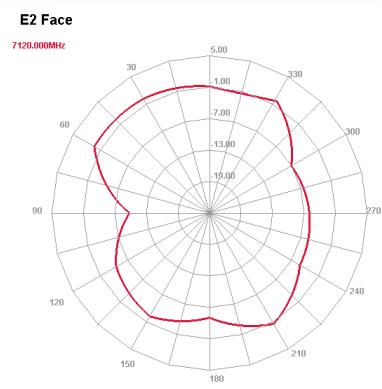
7120 MHz E plane
