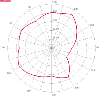
5800 MHz E plane
