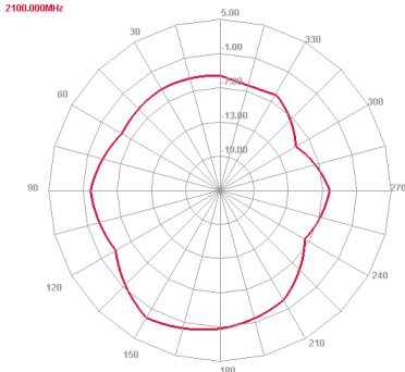
2100 MHz E plane
