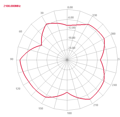
2100 MHz H plane
