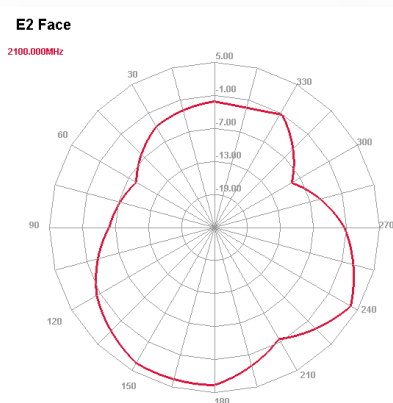
2100 MHz E plane
