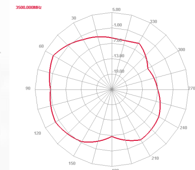
3500 MHz E plane
