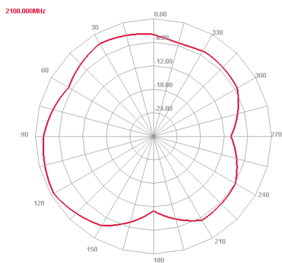
2100 MHz E plane
