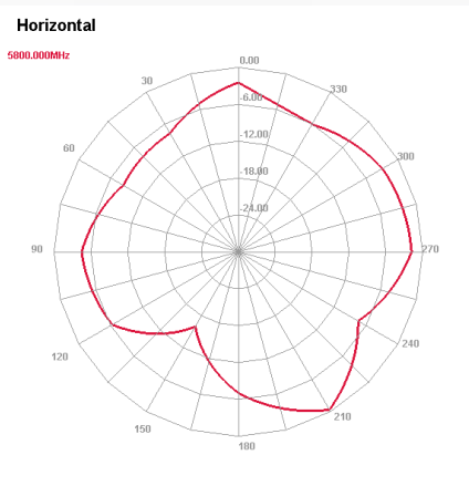
5800 MHz H plane
