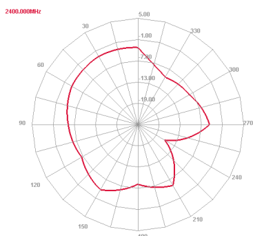
2400 MHz E plane
