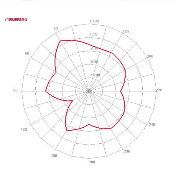
E plane
