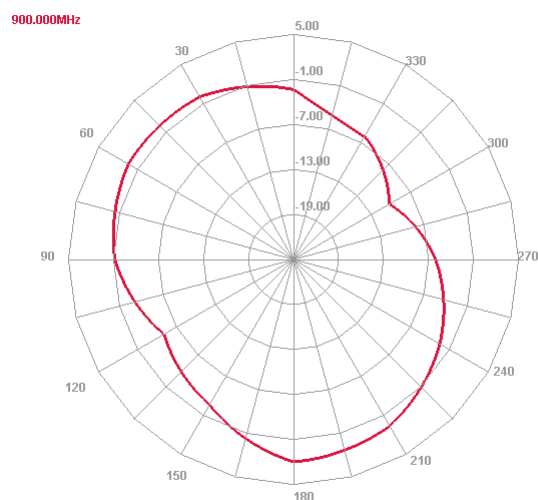
E plane
