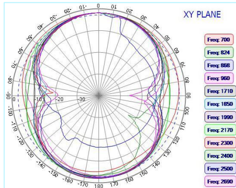
LTE Antenna MAIN part Pattern
