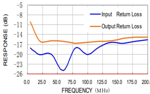
at +12V Pin= -20dBm
