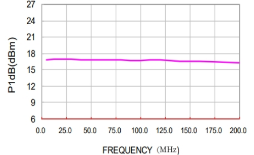
at +12V P1dB
