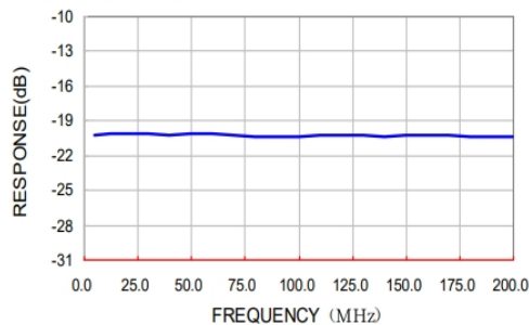
at +12V Pin= -20dBm — S12
