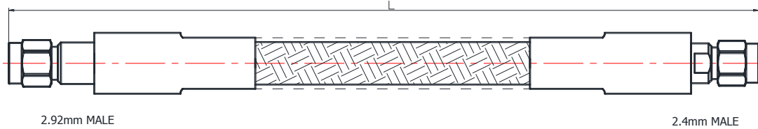
2.92mm MALE
