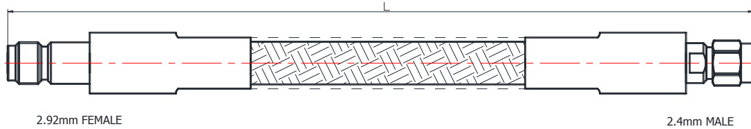
2.92mm FEMALE
