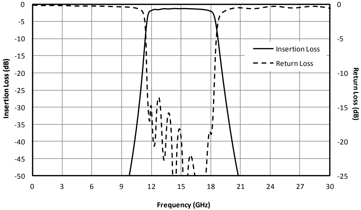
Fig. 1. Magnitude response for a typical FB-1500.
