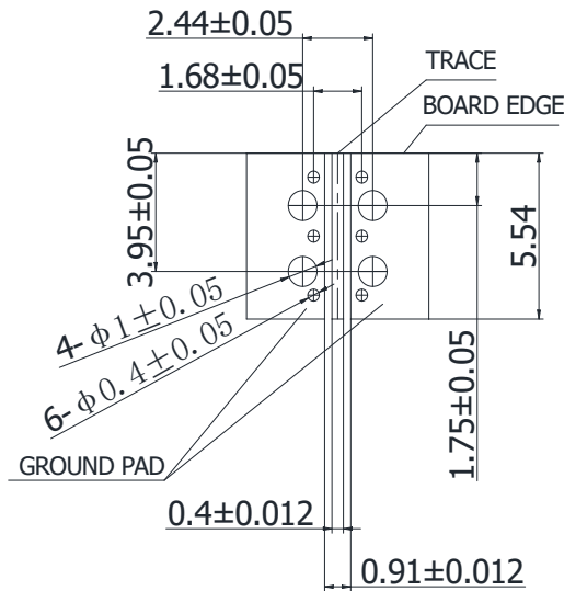
MOUNTING FOOTPRINT
