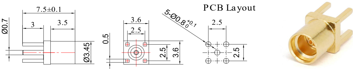
Dimensions are in mm
