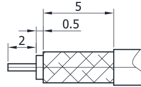
Recommended Cable Stripping Dimension
