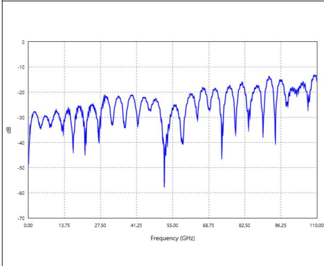
S11 FORWARD REFLECTION
