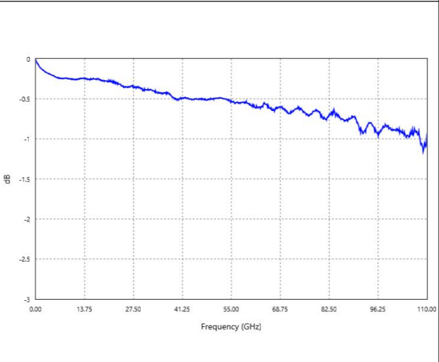
S21 FORWARD TRANSMISSION
