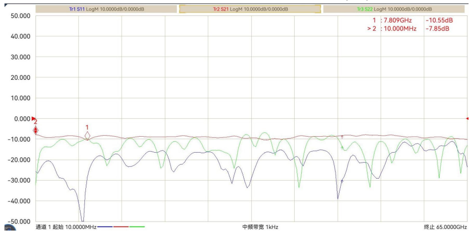
S31 Insertion Loss and Return Loss (dB)
