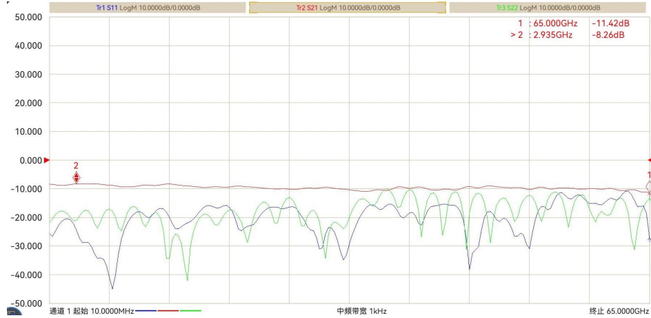
S21 Insertion Loss and Return Loss (dB)
