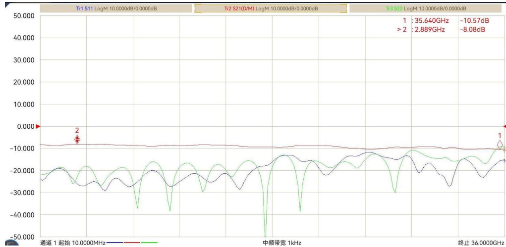
S31 Insertion Loss and Return Loss (dB)
