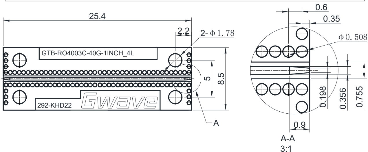
CPWG RO4003C PCB LAYOUT
